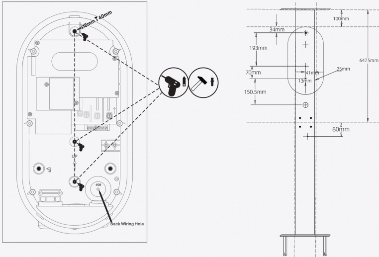
Figure 2-4 Locate the installation location for pole-mounted
